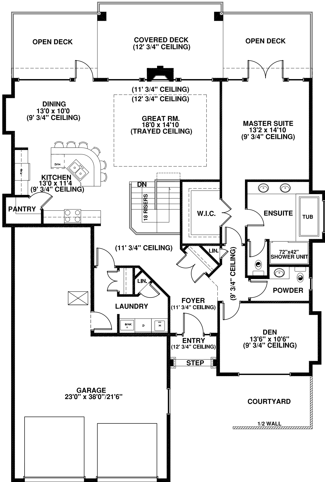
MAIN FLOOR - 1710 SQ.FT.
